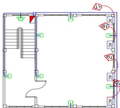
SECOND FLOOR PLAN SCALE 1:100
