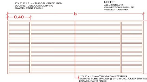
DETAILS OF WINDOWS GRILLS SCALE 1:20
