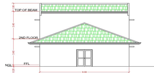
REAR ELEVATION SCALE 1:100
