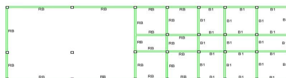
BEAM DESIGNATION @3.40 m SCALE 1:200
