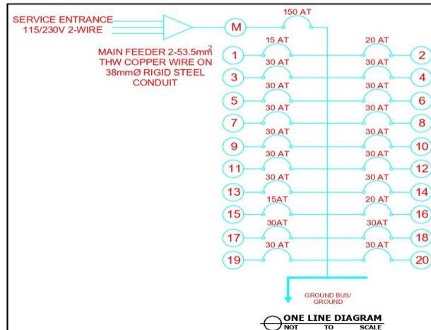
SCHEDULE OF LOADS
