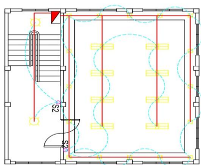
SECOND FLOOR PLAN SCALE 1:100
