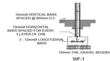
WALL FOOTING DETAILS SCALE NTS
