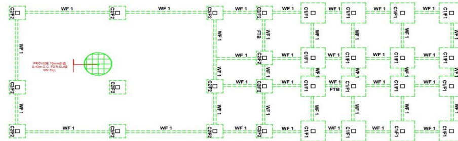
FOUNDATION PLAN SCALE 1:150
