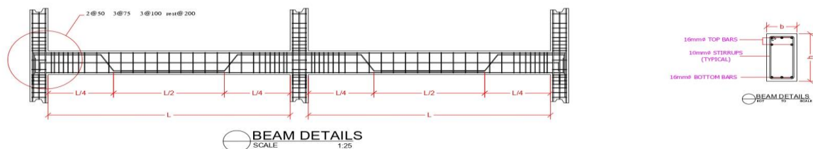
SCHEDULE OF BEAM REINFORCEMENT
