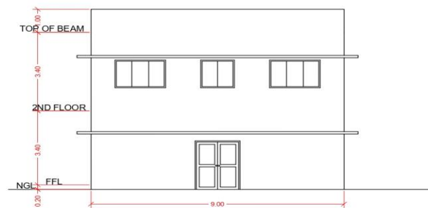
FRONT ELEVATION SCALE 1:100
